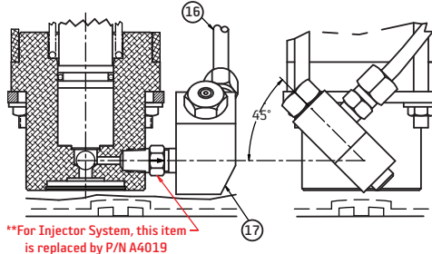
VIEW C – SOLENOID VALVE
