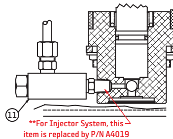
VIEW C – SOLENOID VALVE
