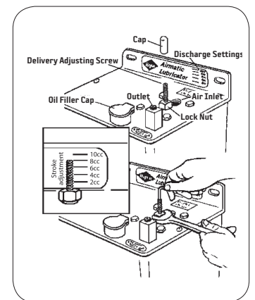
Figure 1: Lubricant Delivery Adjustment
